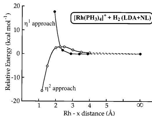
Fig. 7 Reaction profiles for the \eta^1 and \eta^2 approaches of \text{H}_2 towards singlet [\text{Rh}(\text{PH}_3)_4]^+ (LDA + NL)
