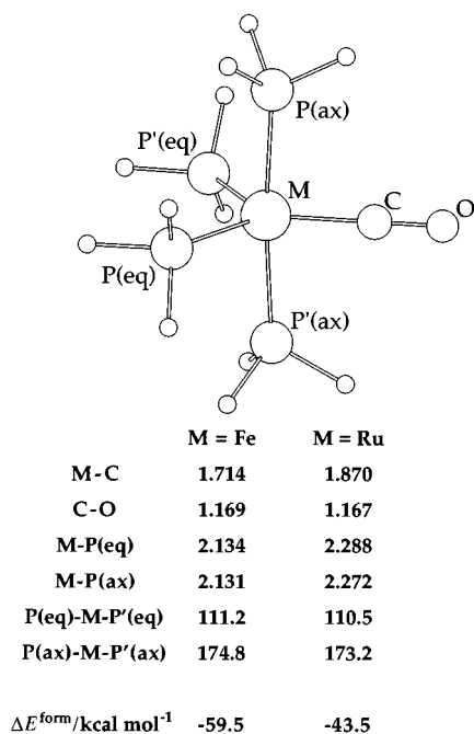
Fig. 9 Geometries of [\text{M}(\text{PH}_3)_4(\text{CO})] species ( \text{M} = \text{Fe} or \text{Ru} )
